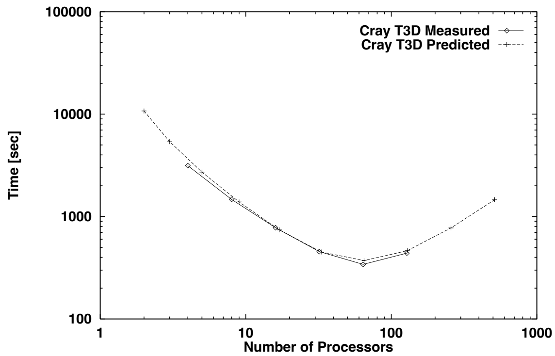
Figure 1c. Actual versus predicted wall-clock time for the CIT AQM.
