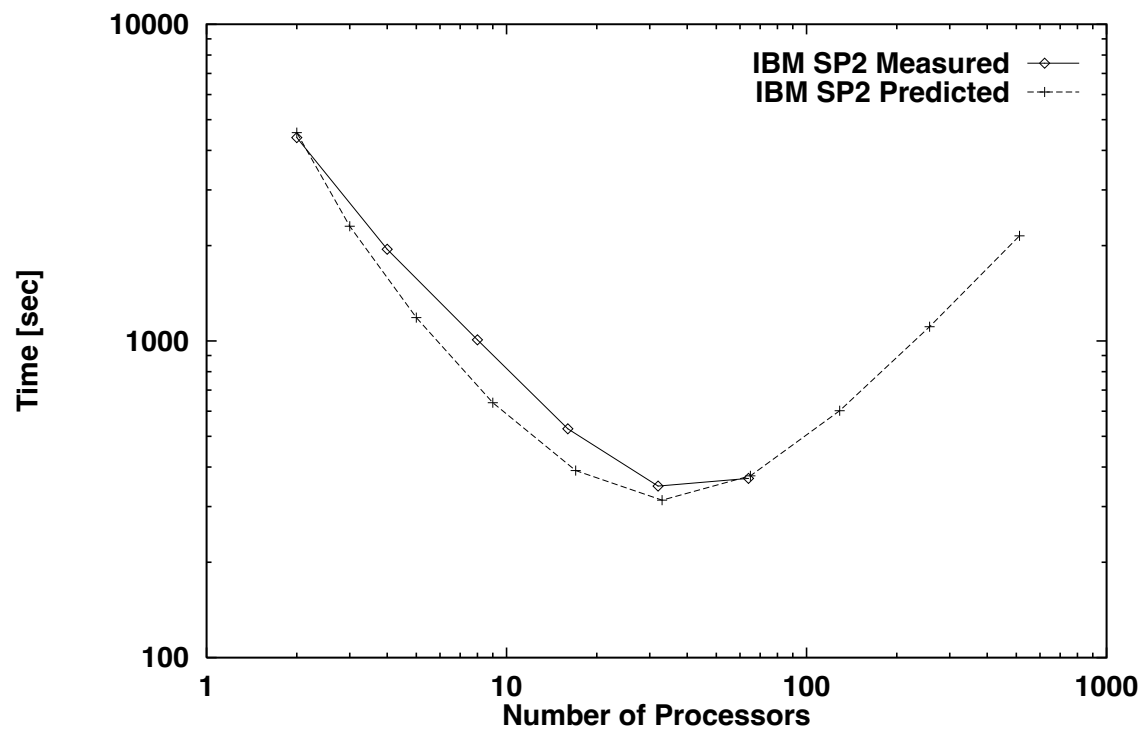
Figure 1d. Actual versus predicted wall-clock time for the CIT AQM.
