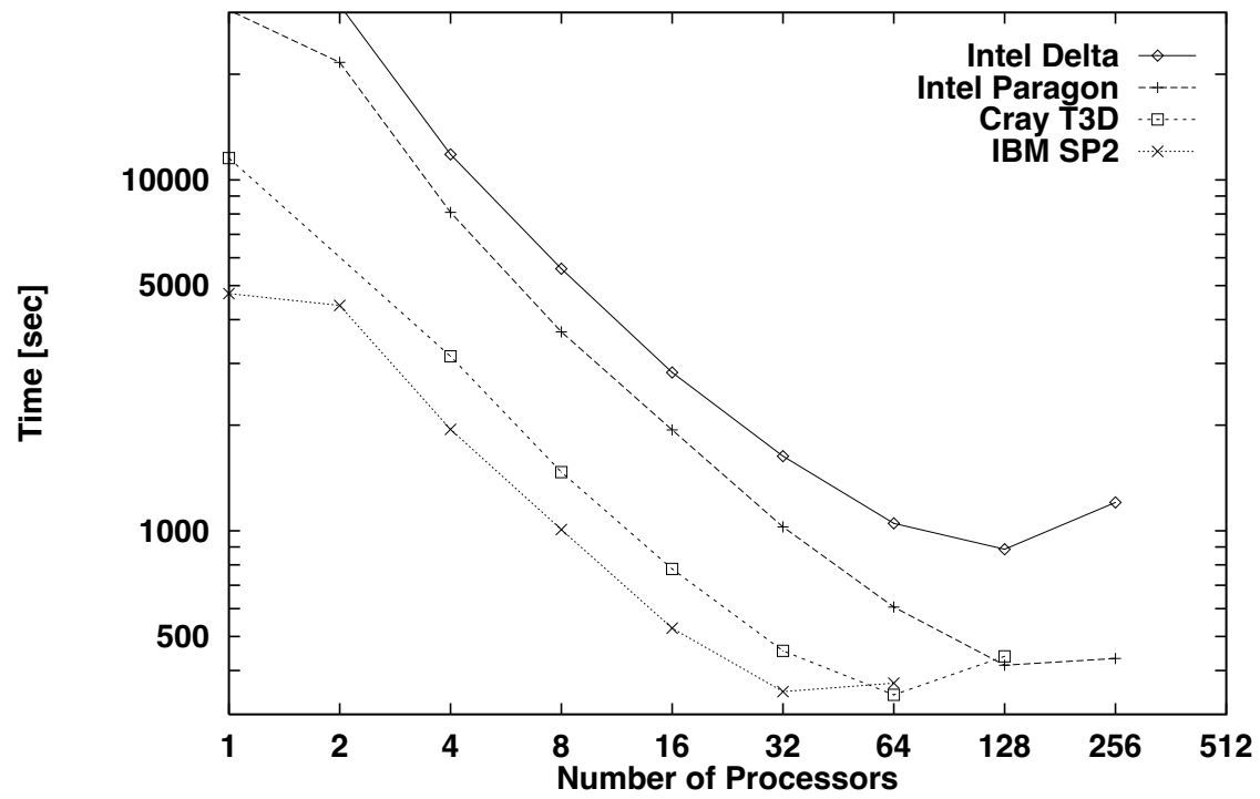
Figure 2. Performance of the parallel CIT AQM on various machines.
