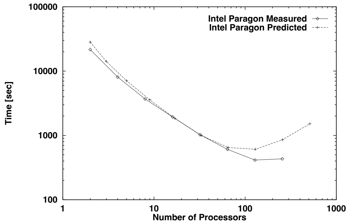
Figure 1b. Actual versus predicted wall-clock time for the CIT AQM.
