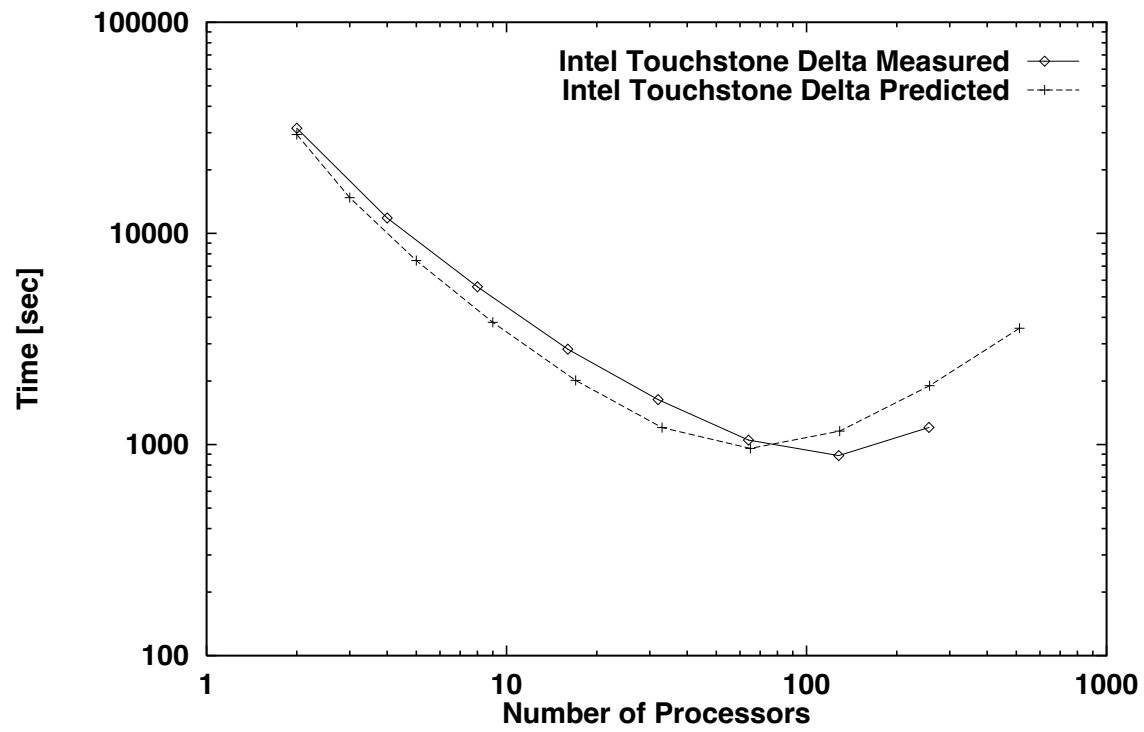
Figure 1a. Actual versus predicted wall-clock time for the CIT AQM.
