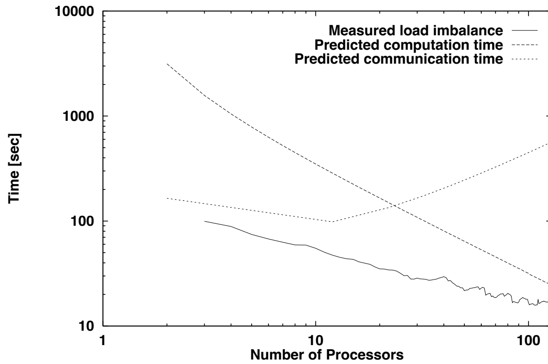
Figure 3. Measured load imbalance, predicted computation and predicted communication times on an IBM SP2.
