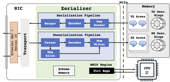
Figure 3: A diagram of the Zerializer architecture and how it is integrated into the NIC.
